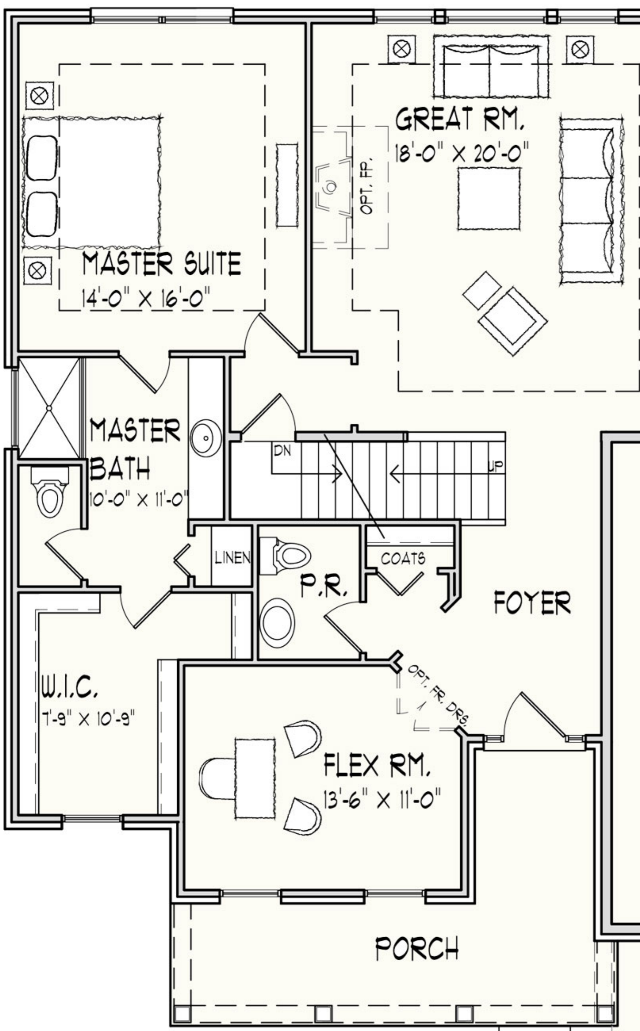
NANTUCKET - FIRST FLOOR
